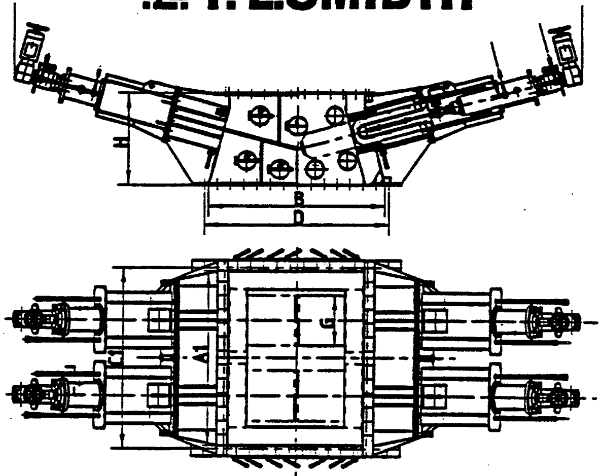
ADJUSTABLE KILN ORIFICE
